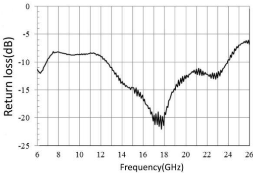
Rf return loss
