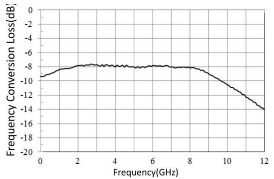
IF bandwidth @LO=26GHz, LO=13dBm
