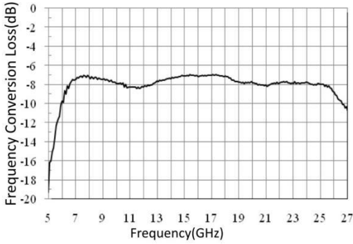
Frequency conversion loss curve @LO=13dBm, IF frequency 0.5GHz
