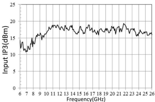
Input IP3@LO=13dBm
