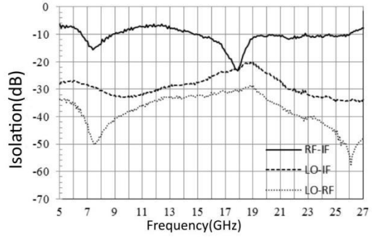
isolation @LO=13dBm, if frequency 0.5GHz
