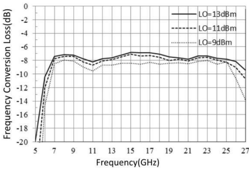
Frequency conversion loss curve @ IF frequency 0.5GHz
