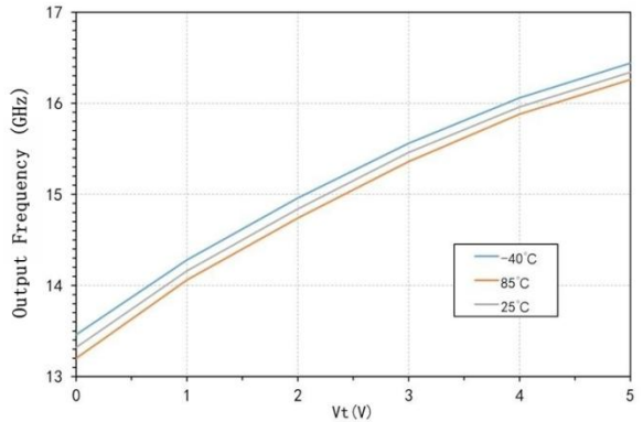
RFOUT output frequency VS Vt @ band 9
