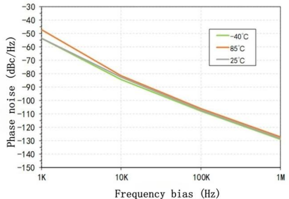
Phase noise vs. frequency bias @ Vt=3V@band 9
