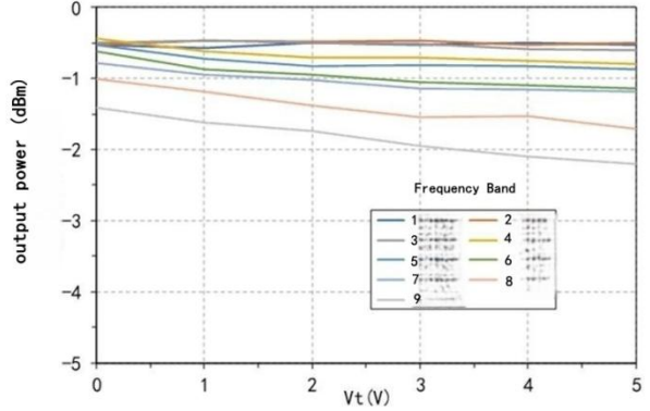
RF/N output power VS Vt (N=8)
