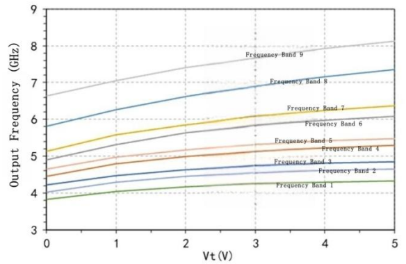
RF/N output frequency VS Vt (N=8)
