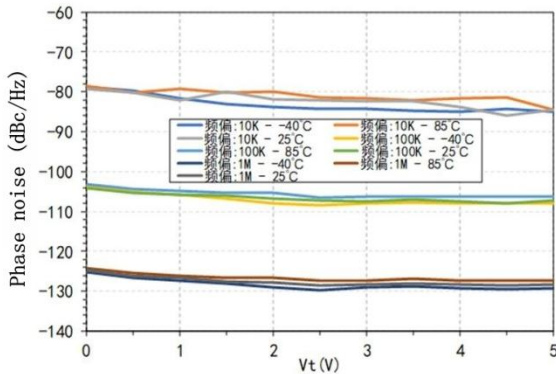
Phase noise VS Vt @ band 9
