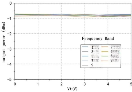
RF/N output power VS Vt (N=16)
