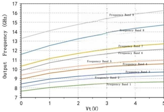
RF/N output frequency VS Vt (N=4)
