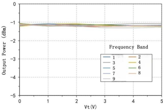
RF/N output power VS Vt (N=16)
