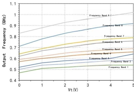
RF/N output frequency VS Vt (N=16)
