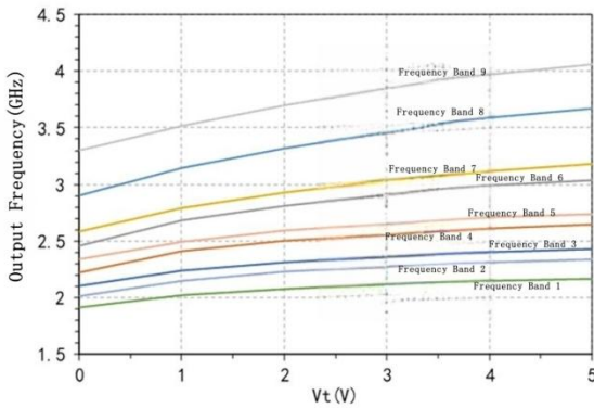
RF/N output frequency VS Vt (N=16)
