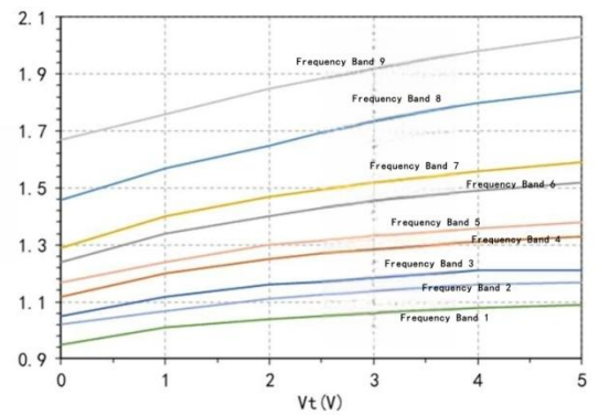
RFOUT tuning sensitivity VS Vt
