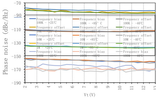
RFOUT phase noise vs. tuning voltage
