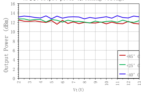
RFOUT output power vs. tuning voltage
