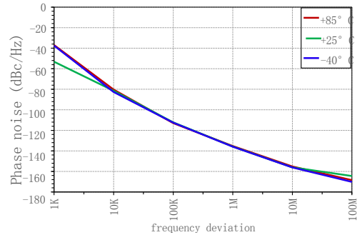
RFOUT phase noise vs. offset frequency @Vt=5V
