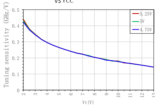
Tuning sensitivity vs VCC
