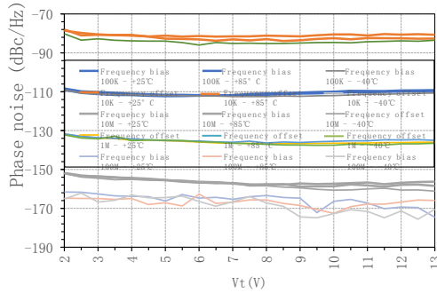
RFOUT phase noise vs. tuning voltage
