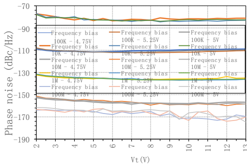
RFOUT phase noise VS VCC
