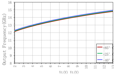
RFOUT output frequency VS tuning voltage
