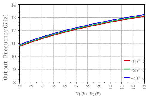
RFOUT output frequency VS tuning voltage
