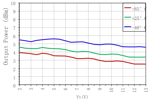
RF/2 output power vs. tuning voltage
