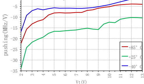
Push factor vs. tuning voltage
