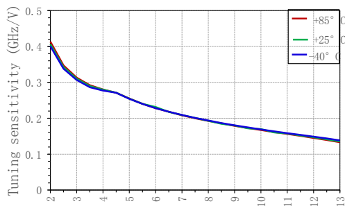
Tuning sensitivity vs. tuning voltage
