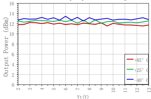
RFOUT output power vs. tuning
