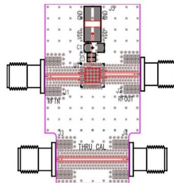
Circuit Board:Rogers4350B
