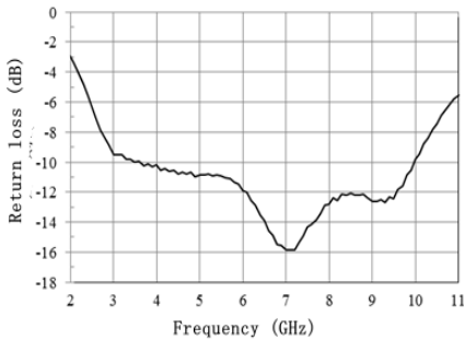
RF return loss
