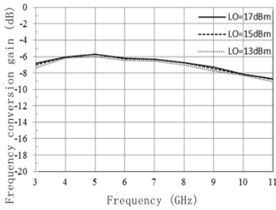
Frequency conversion loss @ IF frequency 0.1 GHz
